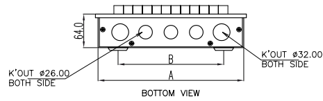
GA DRAWINGS FOR - TPN DB: IPN-30 (Single Door)
