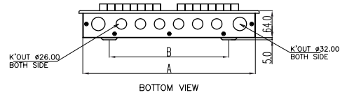
GA DRAWINGS FOR - SPN DB: IP-42 (Double Door)
